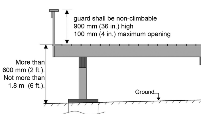
FIGURE 13 - GUARDRAIL HEIGHT
